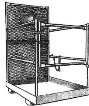
Forklift work platform has standard guardrails and a screen to prevent contact with moving parts of the mast. A chain secures the platform to the mast.
