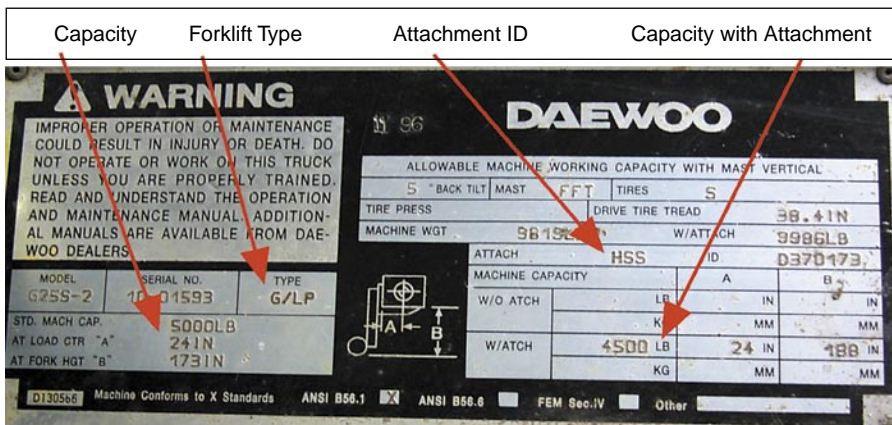
This LP Gas Forklift can safely lift 5000 lbs. 173" high with a center of gravity 24" from the face of the forks. With an attachment labeled "HSS", the safe load drops to 4500 lbs.
